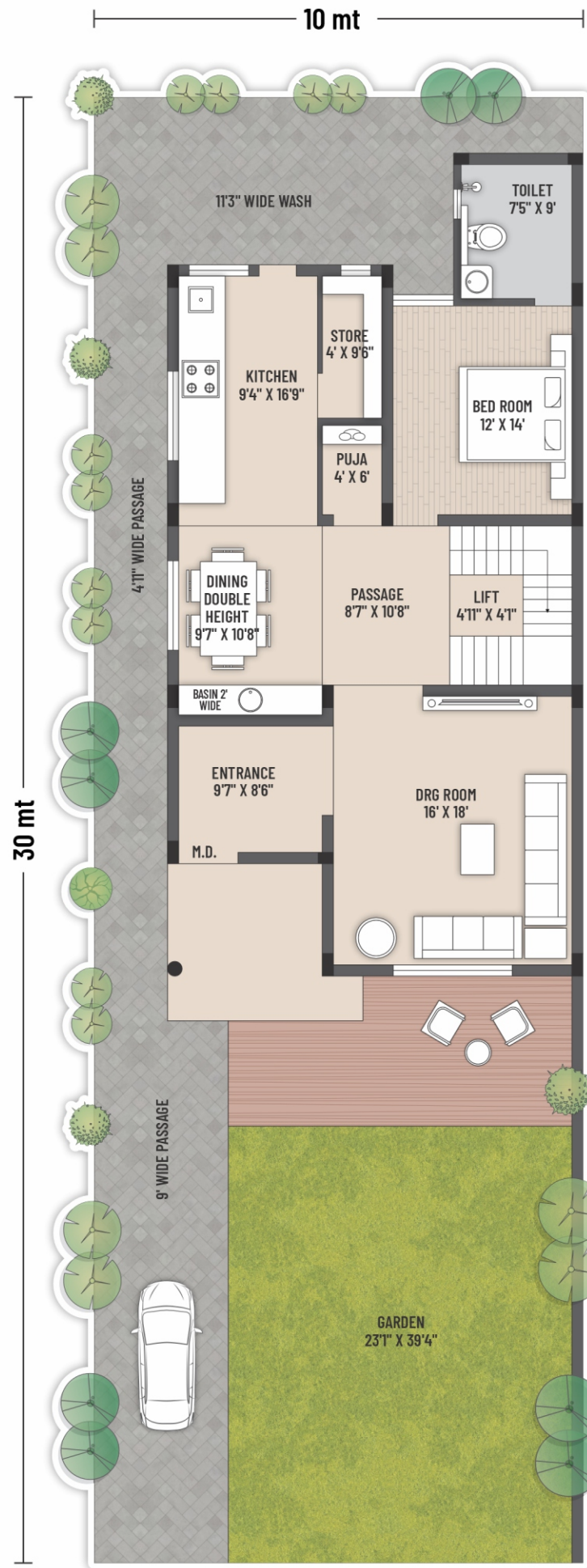
- GROUND FLOOR -
