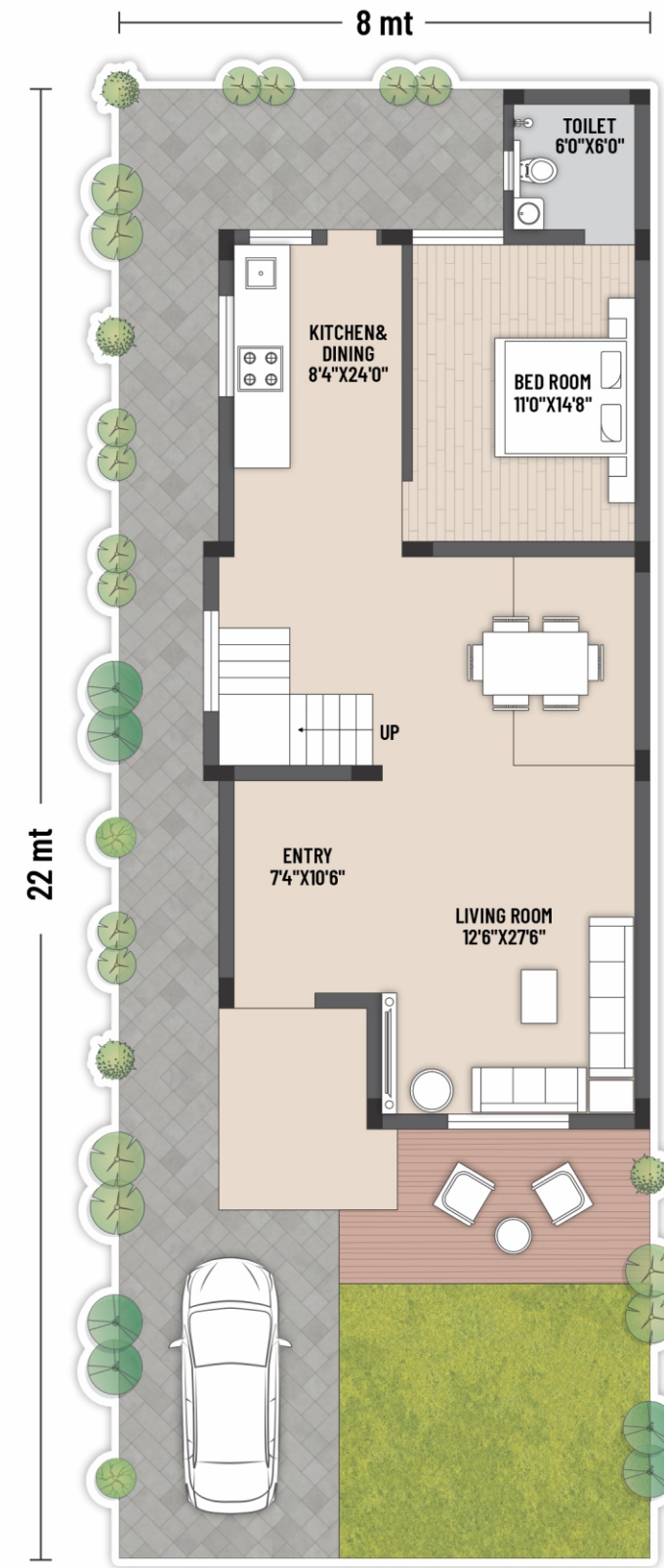
- GROUND FLOOR -
