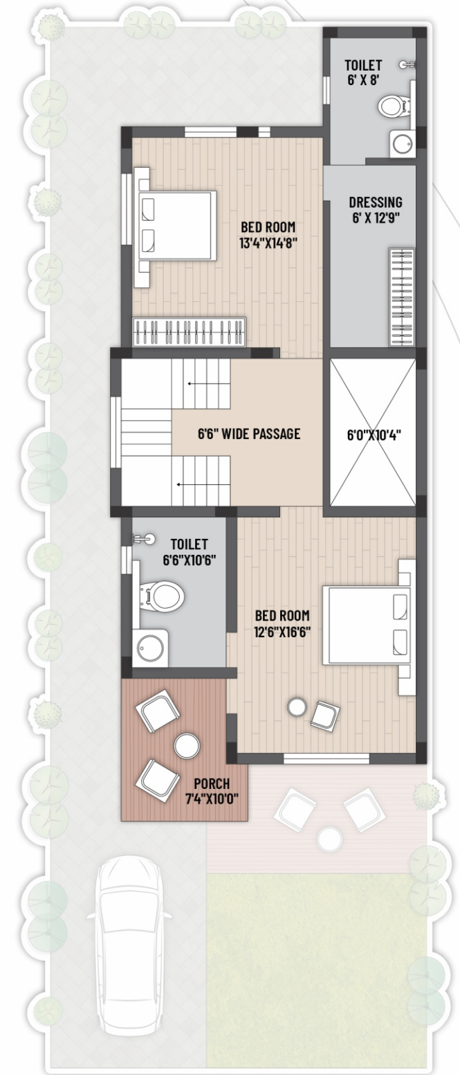
- FIRST FLOOR -
